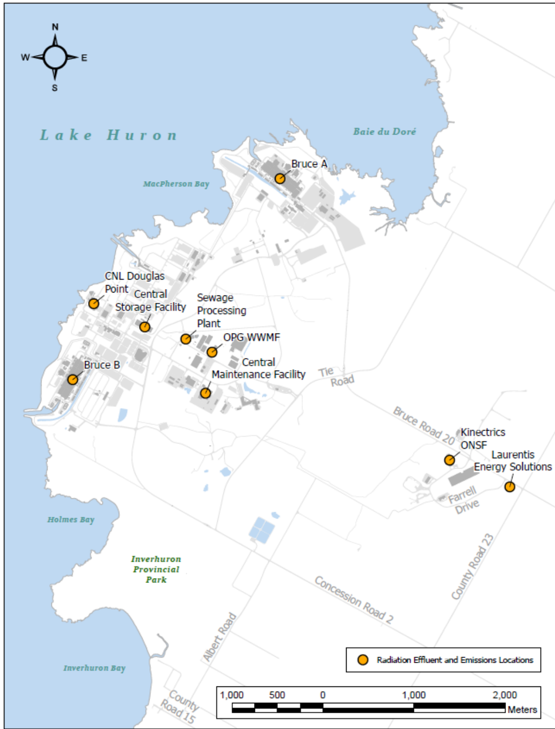
Figure 6 - Radiological Emissions and Effluent Monitoring Locations
